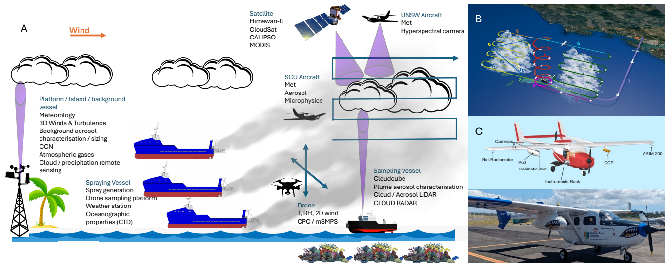
Figure 4: (A) The proposed major field campaign strategy. (B) Flight sampling strategy for aerosol and cloud physics sampling of upwind (background) and downwind (perturbed) cloud. (C) The SCU aircraft 6 .
